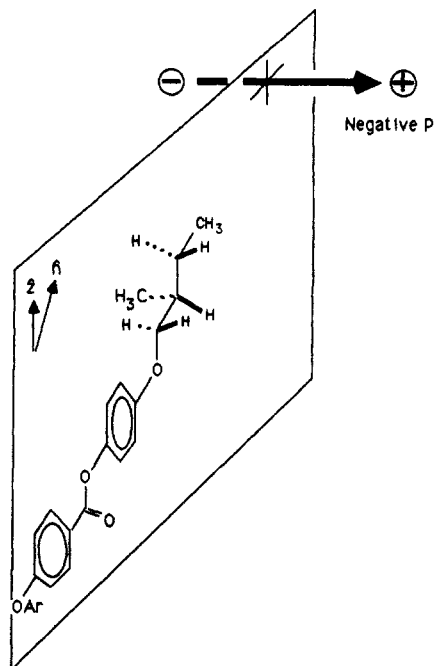
Figure 11. A p -( S )-2-[(methylbutyl)oxy]phenyl benzoate 7 oriented with the butyl chain in the smectic tilt plane. The experimentally determined sign of the polarization is indicated by the P vector in the drawing.
