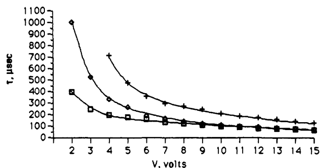
Figure 6. Optical rise times \tau as a function of driving voltage for compound 1 R^1 = n -dodecyl, R^2 = n -propyl ( \square , T = 32.0^\circ\text{C} ), compound 1 R^1 = n -decyl, R^2 = ethyl (+, T = 20.5^\circ\text{C} ), and the 50:50 mixture of these two compounds ( \diamond , T = 25.0^\circ\text{C} ). Measurements were made under conditions identical to those described for Figure 5.
