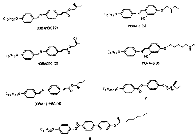
Chart I. Representative Ferroelectric Liquid Crystals
