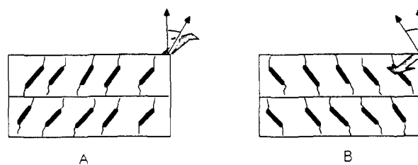
Figure 2. Two stable states of an SSFLC cell.
